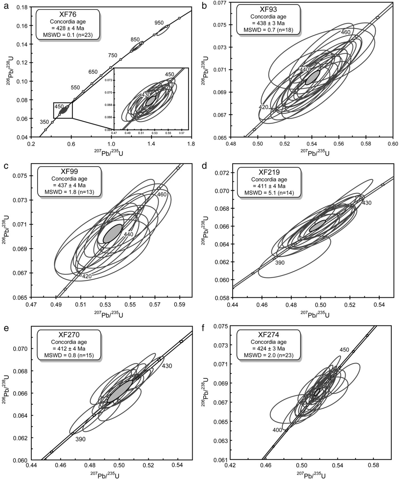
Fig. 5. SIMS U–Pb concordia diagrams of Early Paleozoic granite samples.
