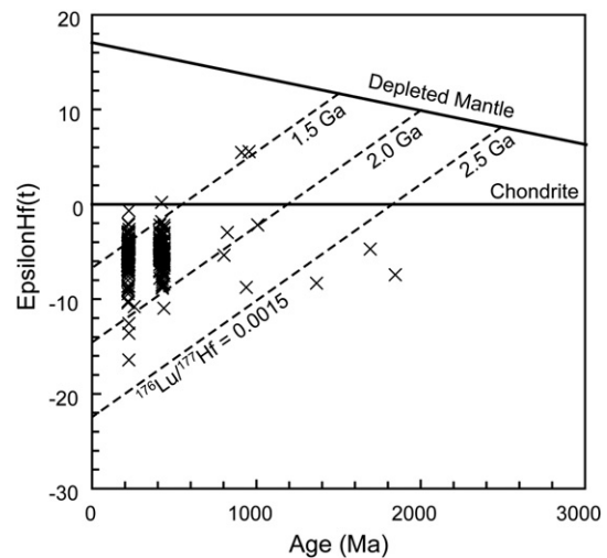
Fig. 8. Diagram of \varepsilon_{\text{Hf}}(t) vs. U–Pb ages of all of zircons from Early Paleozoic and Early Mesozoic granite samples.
