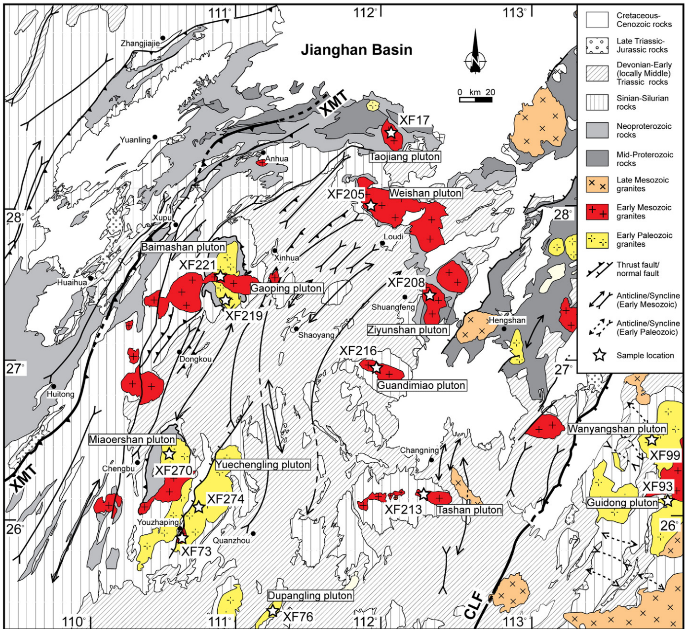
Fig. 2. Geologic map of the Xuefengshan Belt with sample locations of granites XMT: The Xuefengshan Main Thrust. CLF: The Chenzhou-Linwu Fault. (Modified after BGRMGX, 1985; BGRMHN, 1988).
