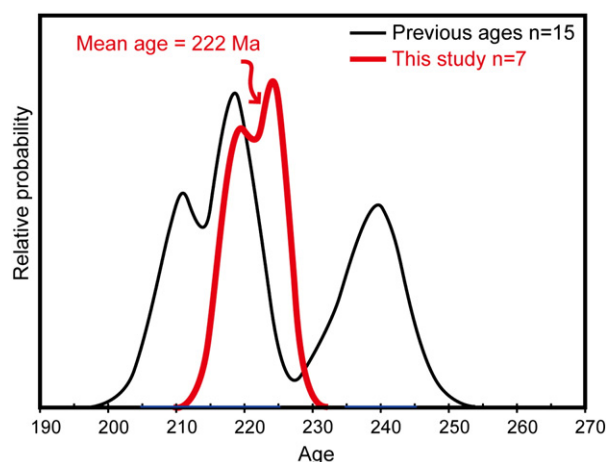
Fig. 9. Relative probability plots of isotopic ages of Triassic granites. Previous age data are from the following references (Chen et al., 2006, 2007a, 2007b; Ding et al., 2005; Li and Li, 2007; Li et al., 2008; Wang et al., 2007a; Xu et al., 2004).
