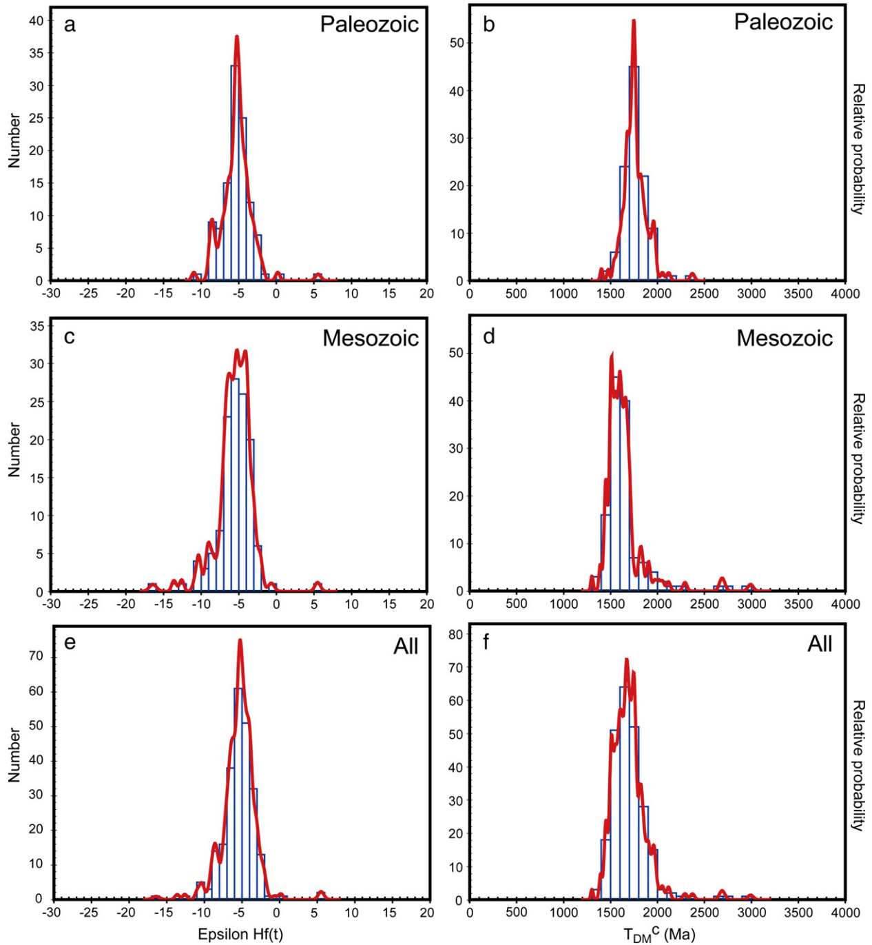
Fig. 7. Diagrams of \varepsilon_{\text{Hf}}(t) and T_{\text{DM}}^{\text{C}} values from Early Paleozoic granites (a–b), Early Mesozoic granites (c–d) and all samples (e–f) in the Xuefengshan Belt.
