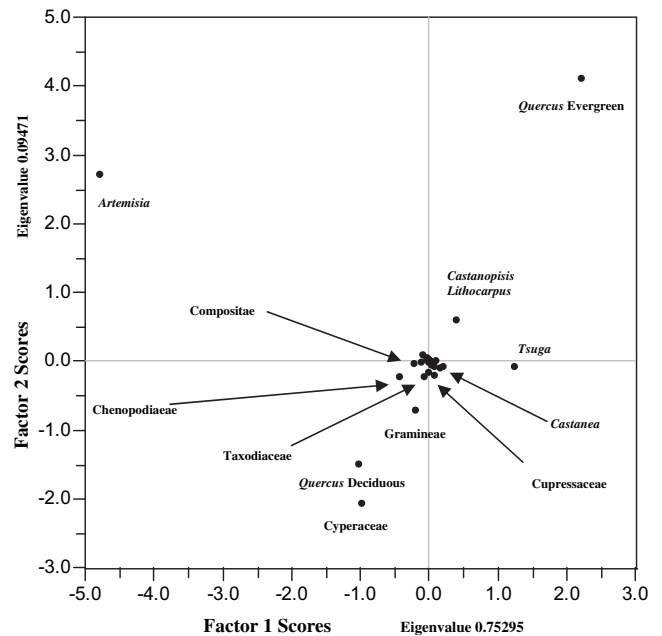
Fig. 4. Principal component analysis of pollen taxa from DG9603 core.
