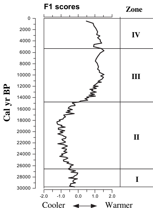
Fig. 5. Variations of factor scores in PCA axis 1.
