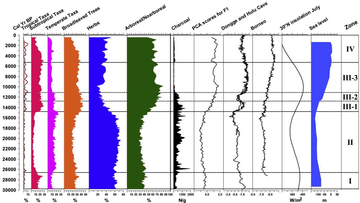
Fig. 6. Multiple records from DG9603 core compared with those of stalagmites and sea-level curve. Stalagmite oxygen isotopic records of Borneo, Dongge Cave and Hulu Cave are from Partin et al. (2007), Wang et al. (2001), and Yuan et al. (2004), respectively. The record of sea-level change in the East China Sea is from Saito et al. (1998).
