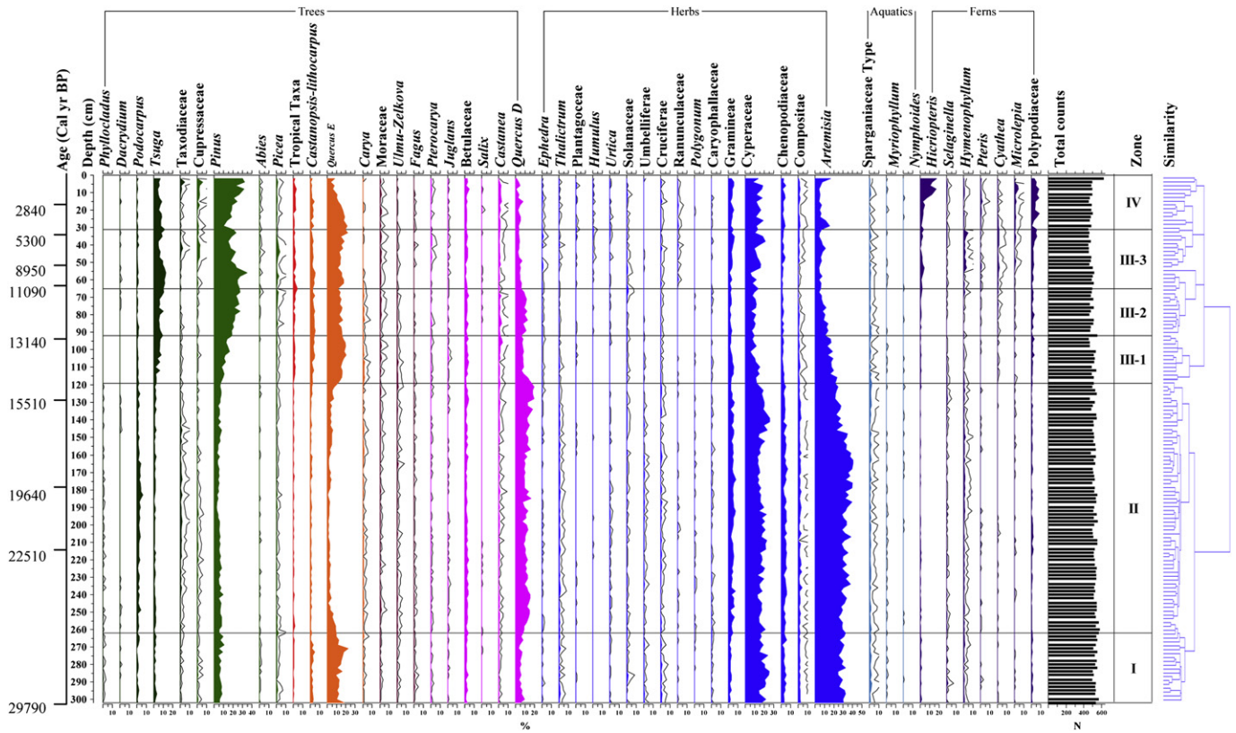
Fig. 3. Analysis of pollen and spore percentage diagram of DG9603 core for the past 30 000 years.
