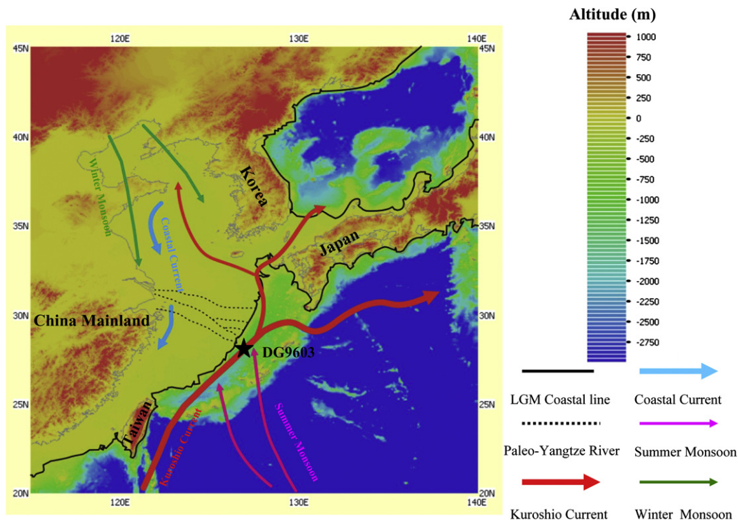
Fig. 1. Location of the studied area and DG9603 core. Paleo-Yangtze River from Xiao et al. (2003) and paleo-monsoon direction after Zhou et al. (2008).
