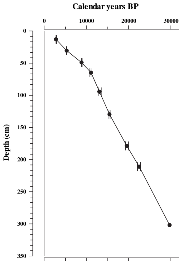
Fig. 2. Age-depth relationship in DG9603 core.
