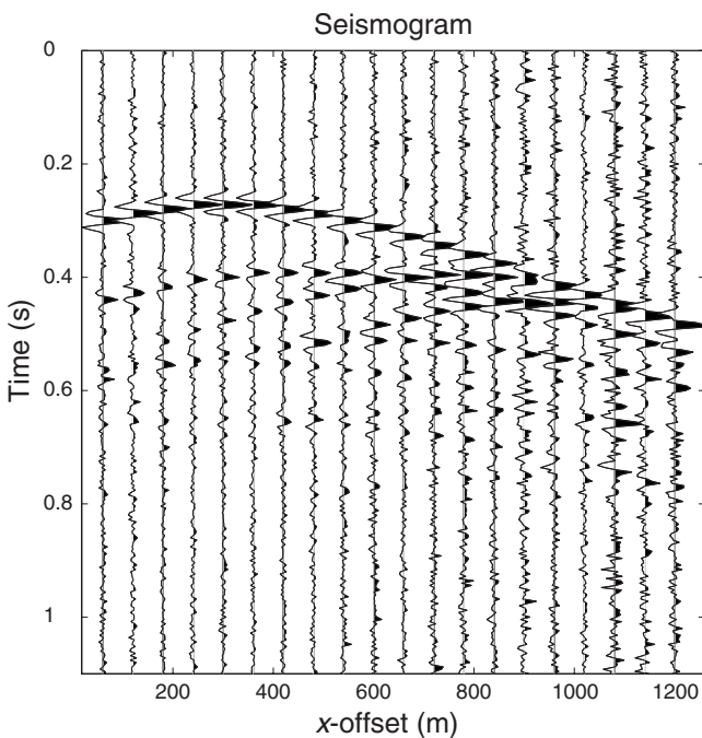
Figure 4. Seismogram from the nine-point scatterer model with noise level equal to 0.005.
