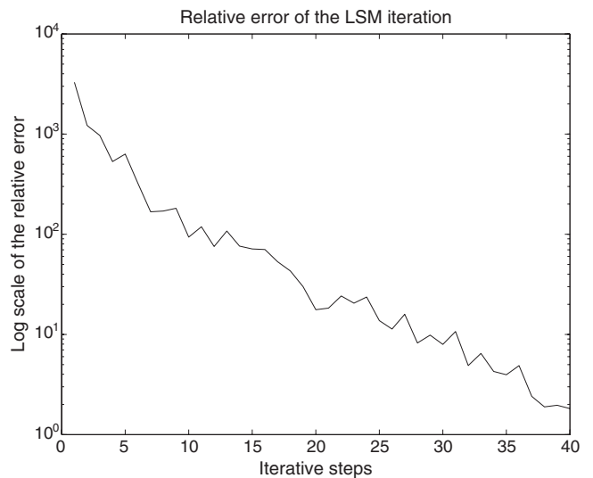
Figure 12. Conjugately monotonic reduction of relative errors of the LSM with noise level equal to 0.01.
