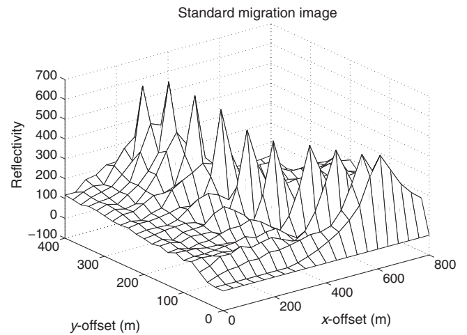
Figure 8. The standard migration image for the ten-point scatterer model with noise level equal to 0.01.
