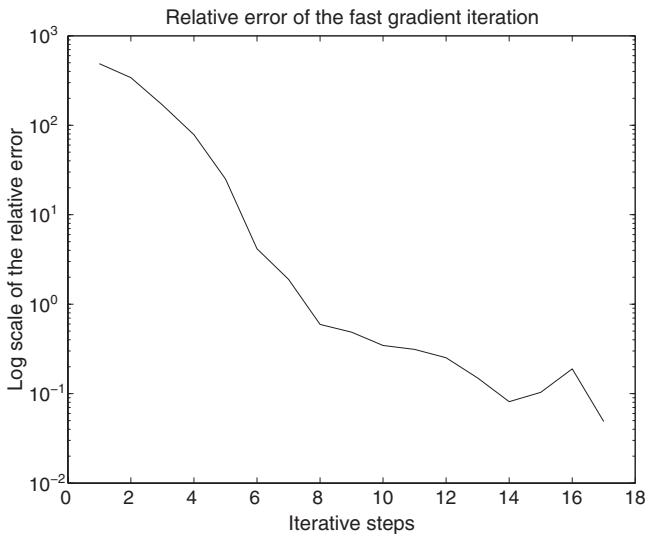
Figure 11. Fast nonmonotonic reduction of relative errors with noise level equal to 0.01.
