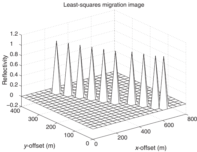
Figure 9. The LSM deconvolution image for the ten-point scatterer model with noise level equal to 0.01.
