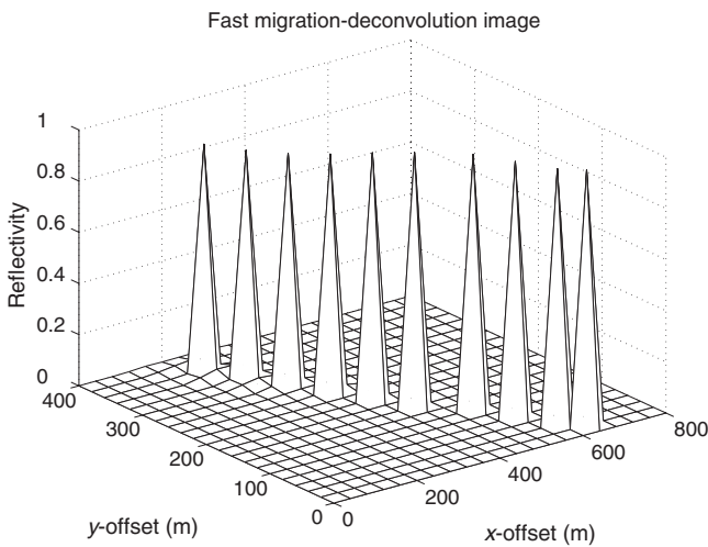
Figure 10. The fast migration-deconvolution image for the ten-point scatterer model with noise level equal to 0.01.
